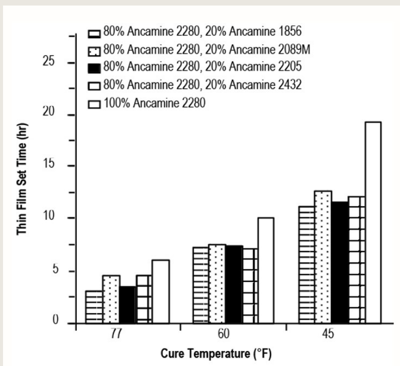
FIGURE 3: CURE SPEEDS OF ACCELERATED ANCAMINE 2280 SYSTEMS
