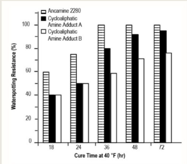
FIGURE 1: WATERSPOTTING RESISTANCE OF CYCLOALIPHATIC AMINE CURING AGENTS
